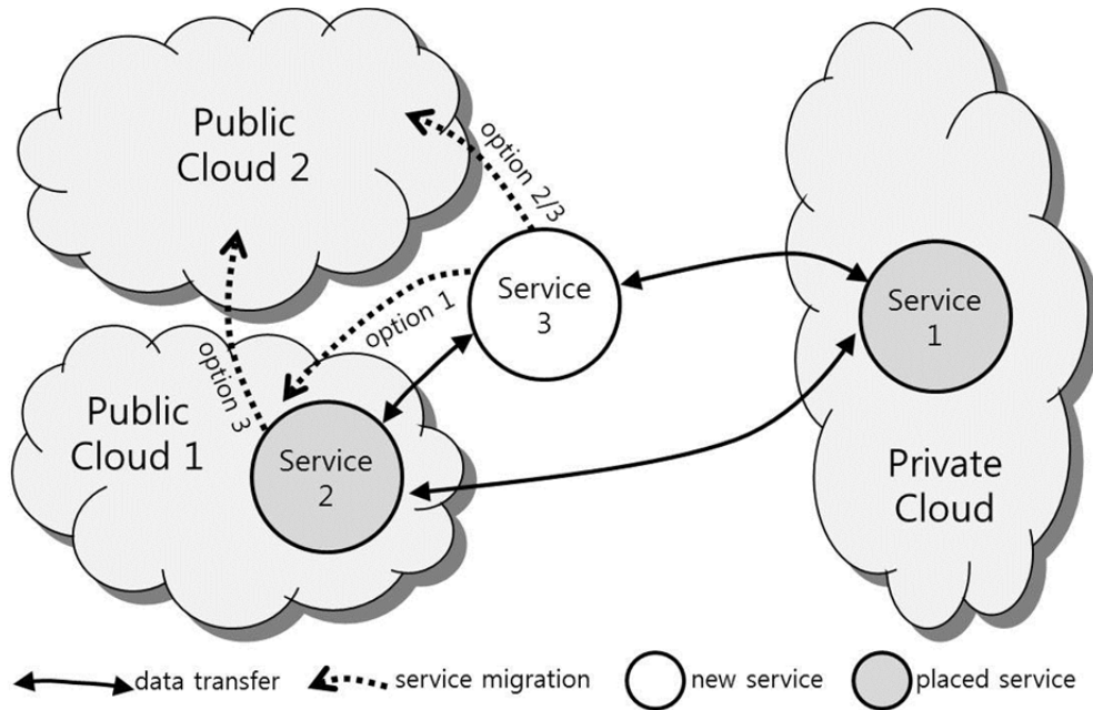
Figure 4. Example of a service placement decision: It is assumed that, initially, service 1 and service 2 run on the private cloud and public cloud 1, respectively. When the demand for service 3 emerges, the company has to decide on a new service placement. There are three service placement options: service 2 and service 3 run on public cloud 1 (option 1), service 2 and service 3 run on public cloud 2 (option 3), or service 2 and service 3 run on public cloud 1 and public cloud 2, respectively (option 2).
