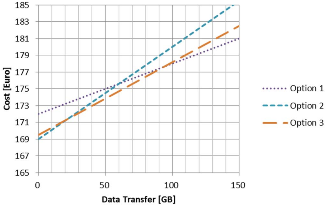
Figure 5. Sensitivity analysis of the three service placement options for the scenario shown in Figure 4. For the comparison, the COMBSPO algorithm is executed with different data traffic matrices. The total traffic is varied from 0 GB to 150 GB.
