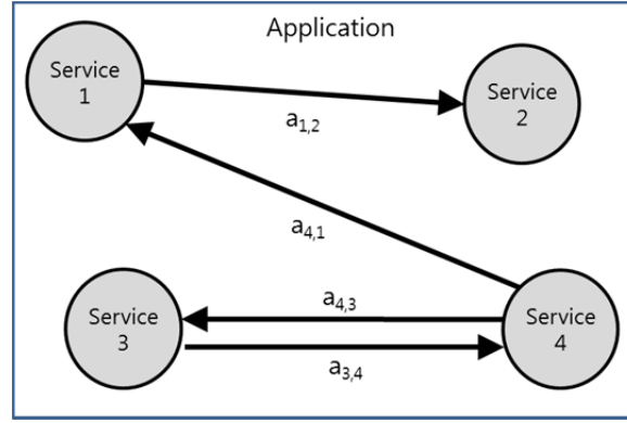
Figure 2. Example of a user application with M=4 services, that exchange data (black arrows).
