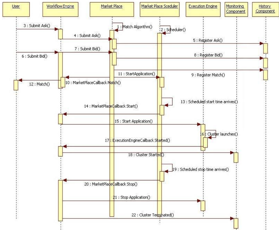
Figure 6. Sequence diagram of implemented services
