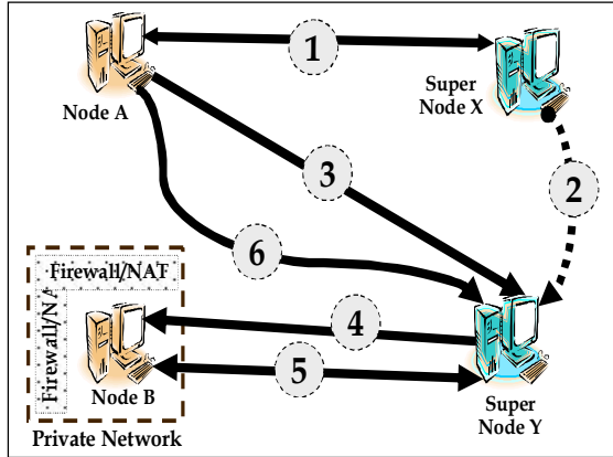
Figure 1. Scenario I: Skype Model
